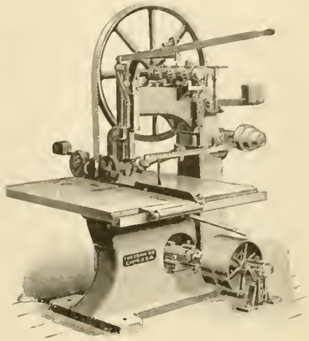
IMPROVED BAND RIP SAW.
